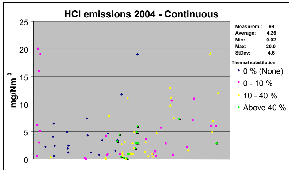
Figure 1.48: HCl emission values from continuous HCl measurement in the clean gas from 98 cement kilns in the EU-27 and EU-23+ countries [97, CEMBUREAU, 2007]
