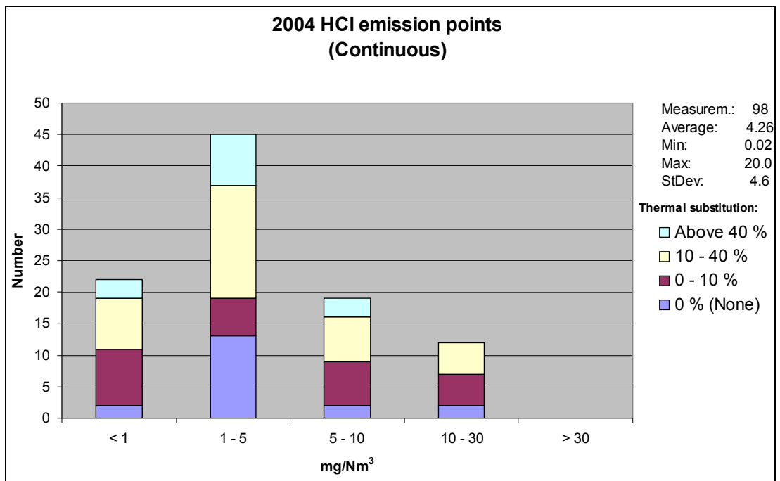
Figure 1.49: Distribution of continuous HCl measurements categorised by the thermal substitution rate [97, CEMBUREAU, 2007]
