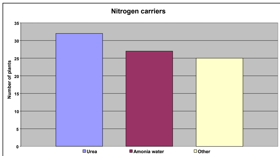
Figure 1.65: Nitrogen carriers/ \text{NH}_2 -X agents used by SNCR in EU-23+ countries [85, CEMBUREAU, 2006]
