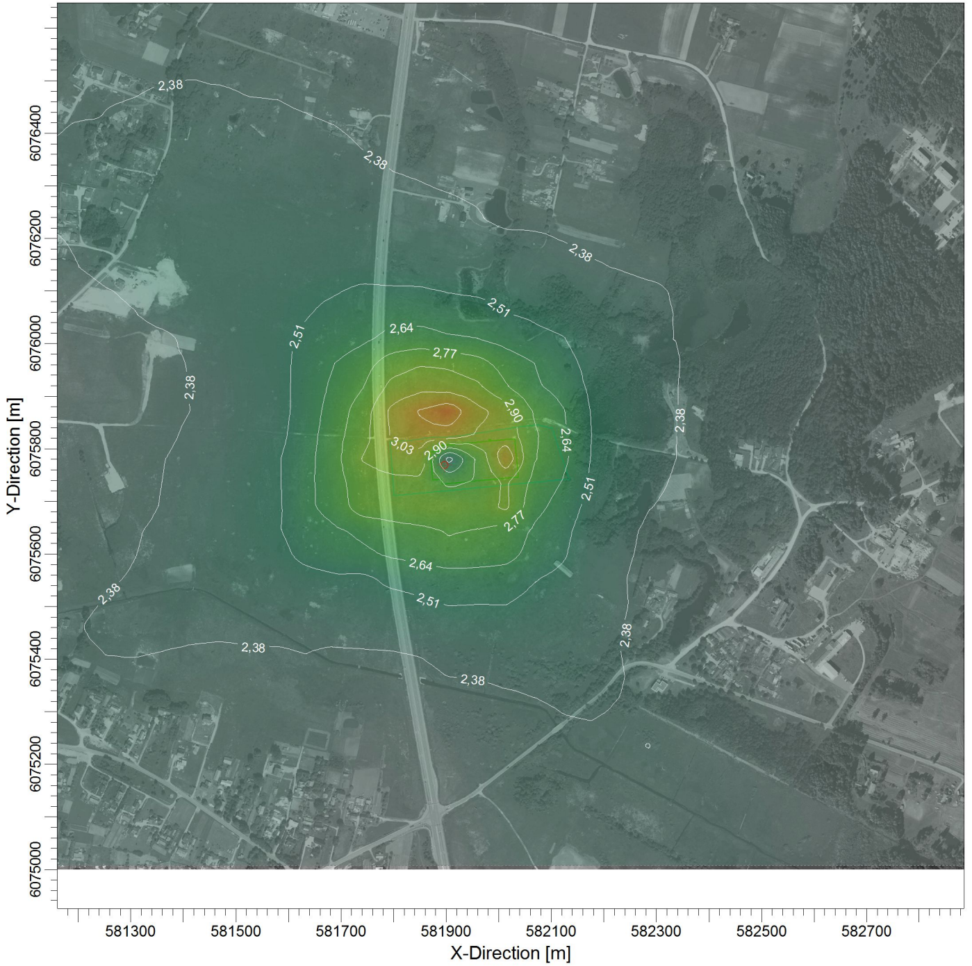
PLOT FILE OF 99.20TH PERCENTILE 24-HR VALUES FOR SOURCE GROUP: ALL Max: 3,42 [ \mu\text{g}/\text{m}^3 ] at (581919,84, 6075853,11)
