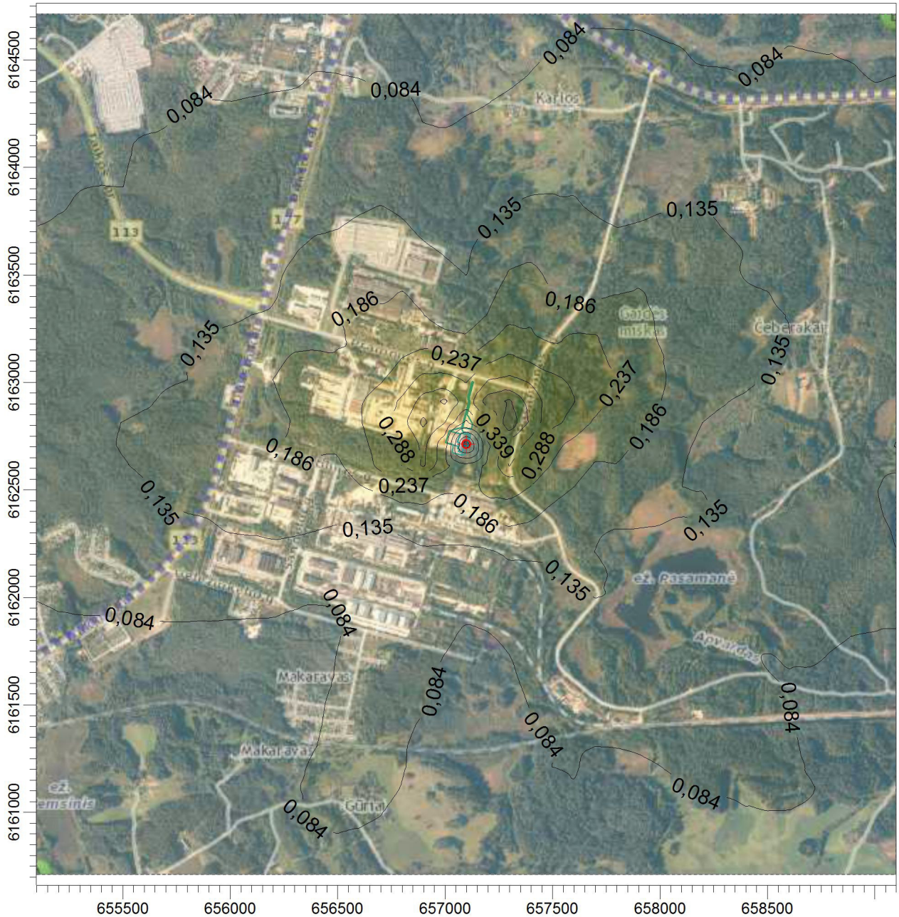
PLOT FILE OF 98.00TH PERCENTILE 1-HR VALUES FOR SOURCE GROUP: ALL
