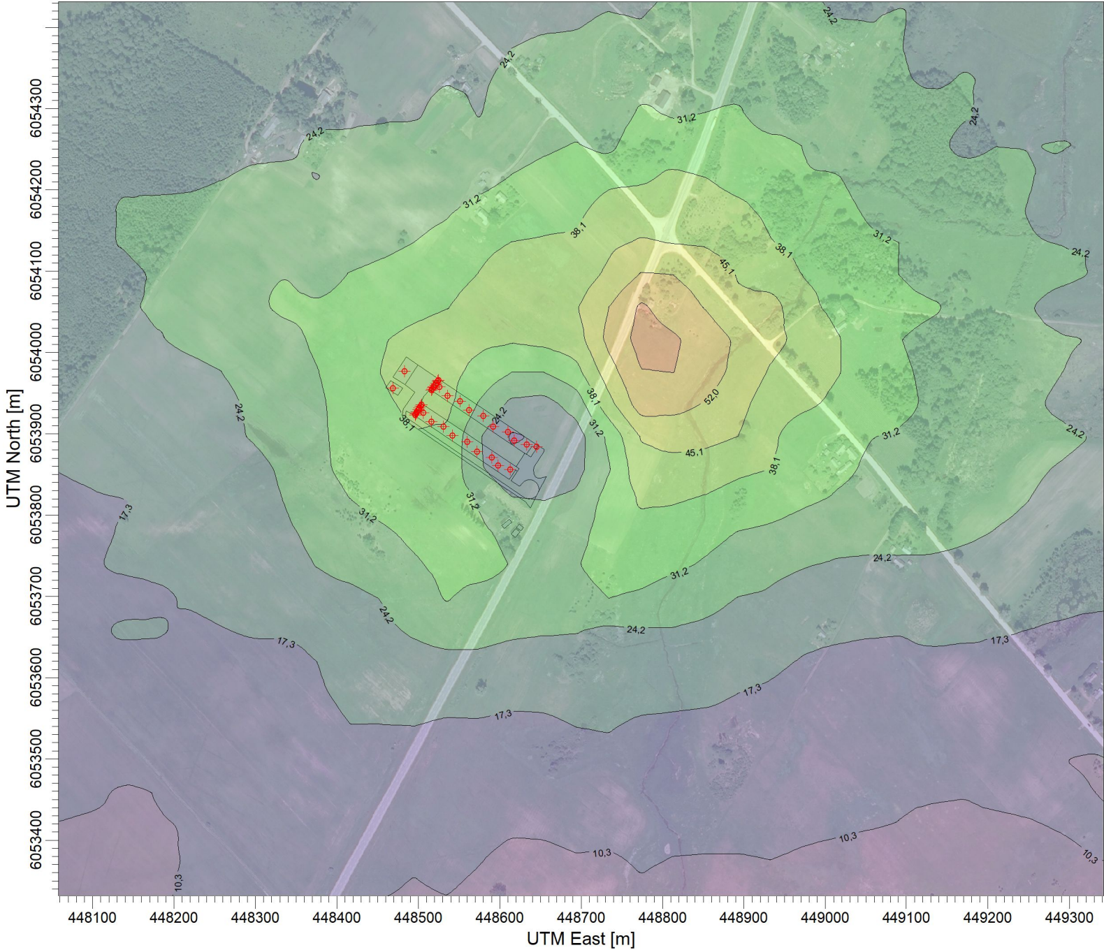
PLOT FILE OF 99.70TH PERCENTILE 1-HR VALUES FOR SOURCE GROUP: SO2 Max: 66,0 [ug/m^3] at (448779,69, 6053952,06)
