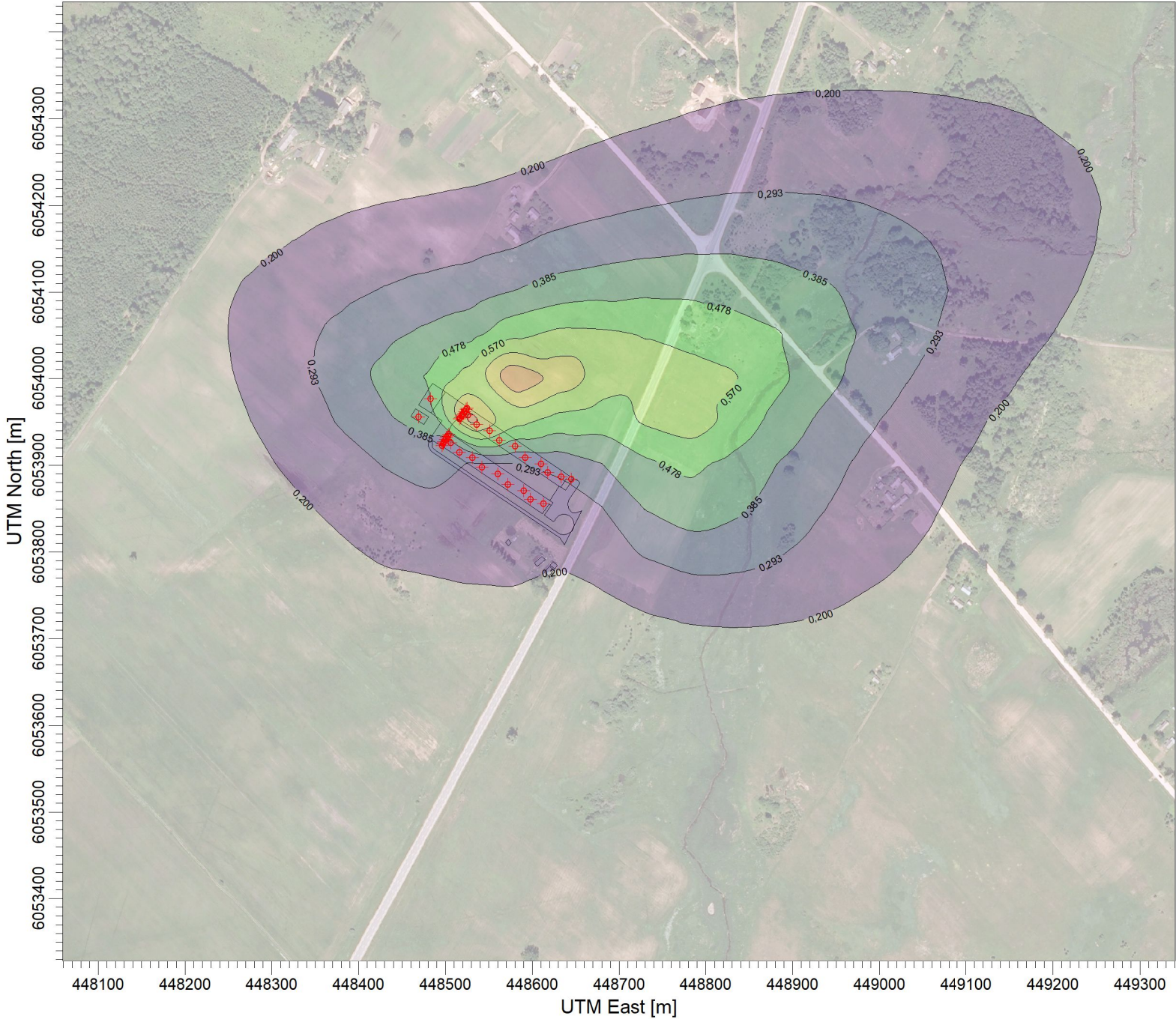
PLOT FILE OF ANNUAL VALUES AVERAGED ACROSS 5 YEARS FOR SOURCE GROUP: PM10
