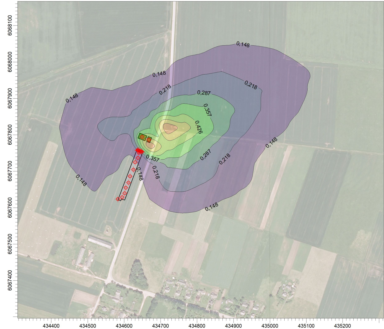
PLOT FILE OF 90.40TH PERCENTILE 24-HR VALUES FOR SOURCE GROUP: PM10
